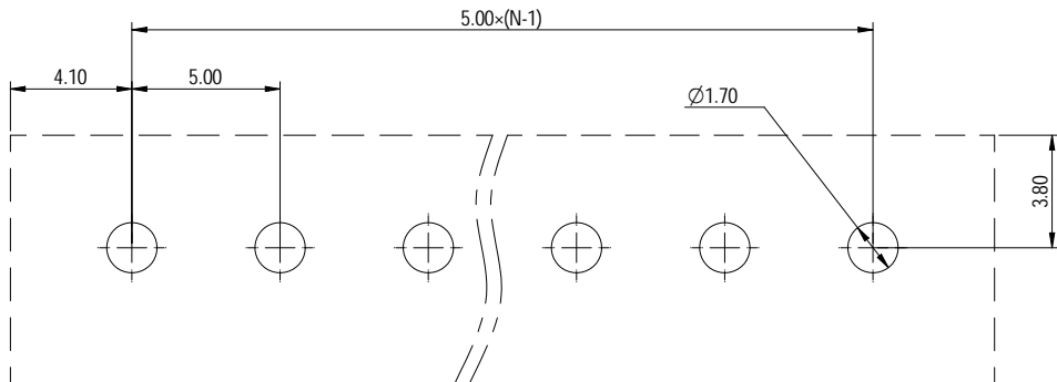
PCB LAYOUT
